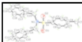
Fig. 1. The molecular structure of the first independent molecule in (I) showing displacement ellipsoids at the 35% probability level.
