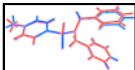
Fig. 3. Overlap diagram highlighting the different conformations of the first (red) and second (blue) independent molecules in (I).
