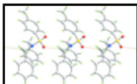
Fig. 4. A view of a supramolecular chain in (I) formed by the first independent molecule aligned along the b axis. The C–H···O contacts are shown as orange dashed lines. Colour code: S, yellow; O, red; N, blue; C, grey; and H, green.
